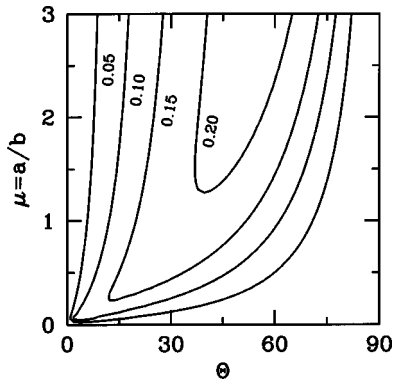
FIG. 3. The normalized amplitude A_{N_t^2}/N^3(A/(a+b)/2)^{-1} for different \Theta and \mu = a/b . Contours are shown by intervals of 0.05, as indicated.
