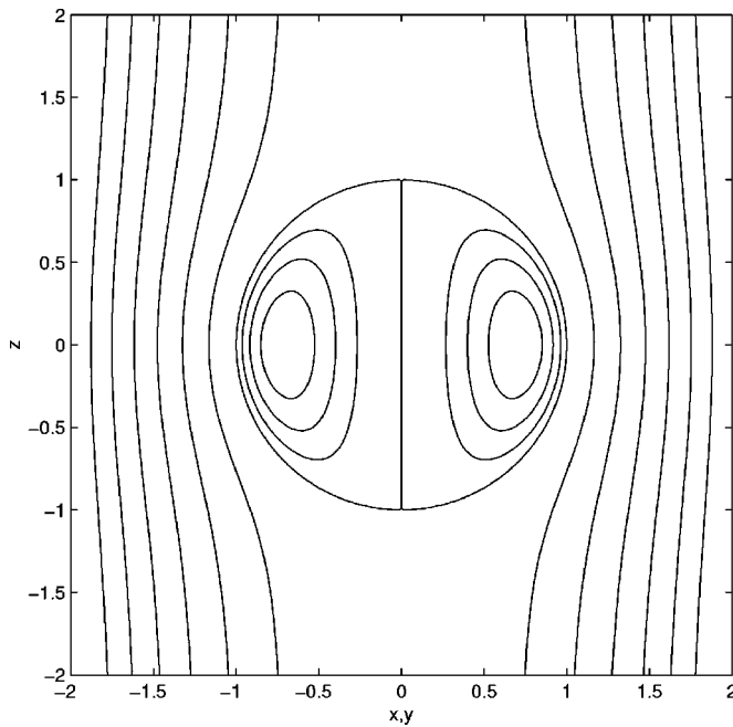
FIG. 1. Streamfunction of HSV in a frame moving with the vortex. The boundary of the vortex corresponds to \psi_0=0 ; the contour values inside are -0.2: 0.05: -0.05 , the contour values outside are 0.25: 0.25: 1.5 .
