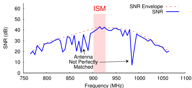
Figure 4: SNR of a tag’s response when the sensing frequency is varied over a wide bandwidth. The SNR (in blue) is consistently higher than 10dB over more than 300 MHz despite that f_s is extremely lower power outside the ISM band.
