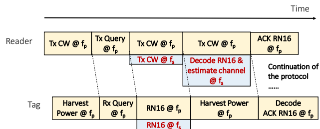
Figure 5: RFind is compatible with the RFID communication protocol. To incorporate RFind into the EPC-Gen2 protocol, a reader only needs to transmit at two frequencies rather than one at the third stage of a communication session.
