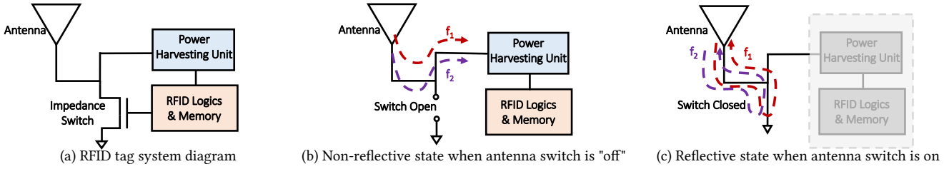
Figure 2: RFID tag antenna impedance control by antenna switch. (a) RFID tag circuit diagram consisting of an antenna, antenna switch, power harvesting unit, and logic & memory circuitry. (b) RFID tag in non-reflective state. Antenna switch is turned "off", resulting in an open terminal. RF power flows into the power harvesting unit. (c) RFID tag in reflective state. Antenna switch is turned "on", resulting in a short terminal. RF power gets reflected by the ground.
