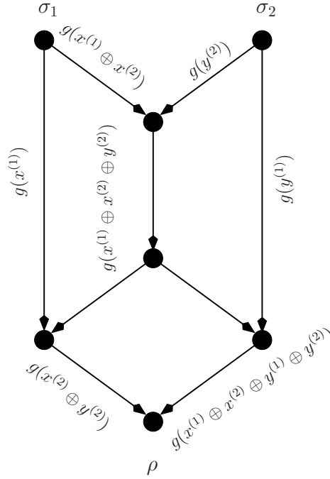
Figure 3.7: The reverse butterfly network with a code that computes the arithmetic sum target function. ‘ \oplus ’ denotes mod 2q - 1 addition.
